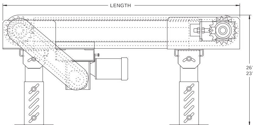
Conveyor shown with optional supports
